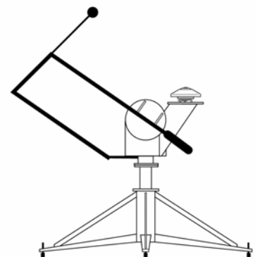
Figure 3 2AP Sun Tracker with shaded pyrometer
