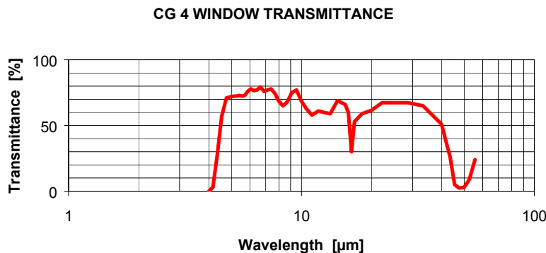
Figure 11 Pyrgeometer spectral window properties
