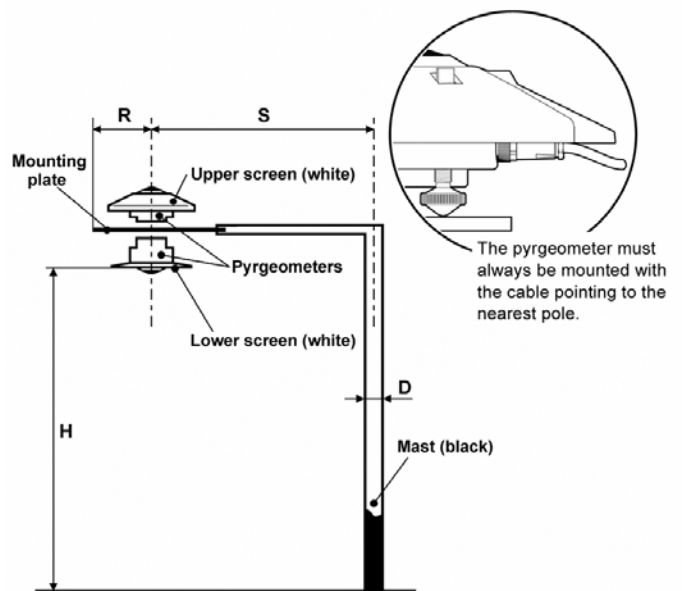
Figure 2 Upward long-wave radiation
