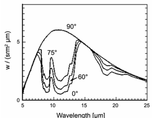
Figure 12 Atmospheric radiation
