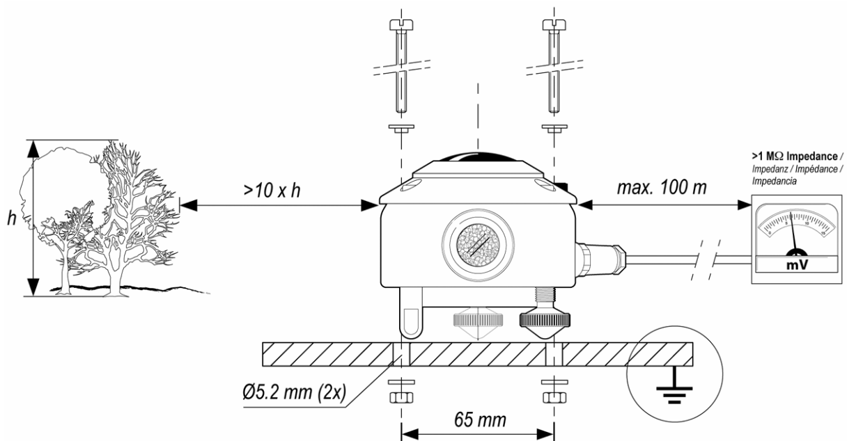
Figure 1 Pyrgometer installation
