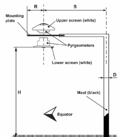
Figure 4 Net radiation configuration
